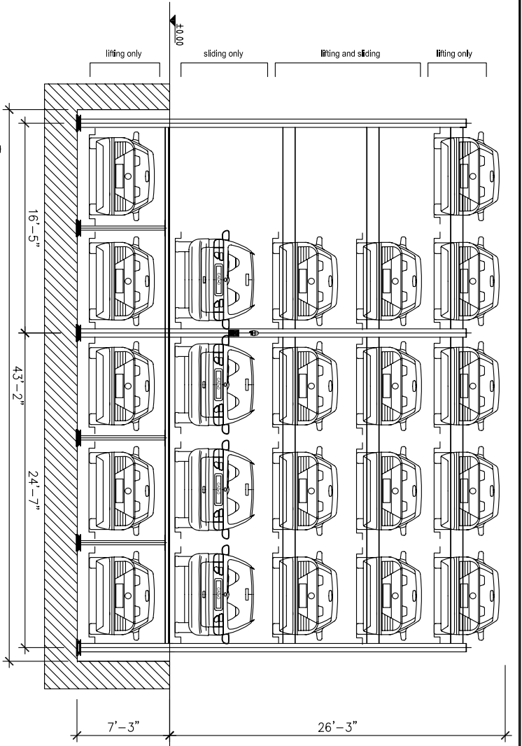
SECTIONAL ELEVATION AA LIFT SLIDING SYSTEM LS4h1d
