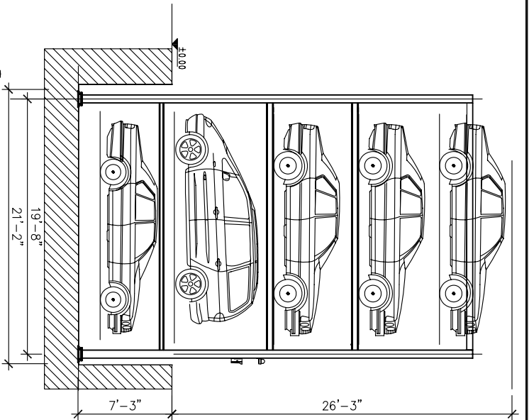
SECTIONAL ELEVATION BB LIFT SLIDING SYSTEM LS4h1d
